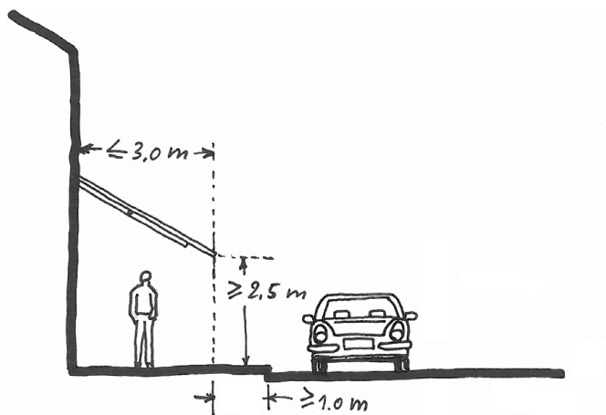
Figure 2 : Saillies mobiles
